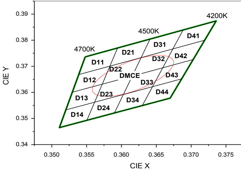
CIE Chromaticity Diagram (Neutral white), T_j=25^\circ\text{C} , I_f=65\text{mA}
