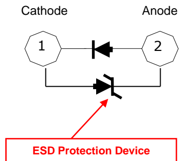
Circuit
