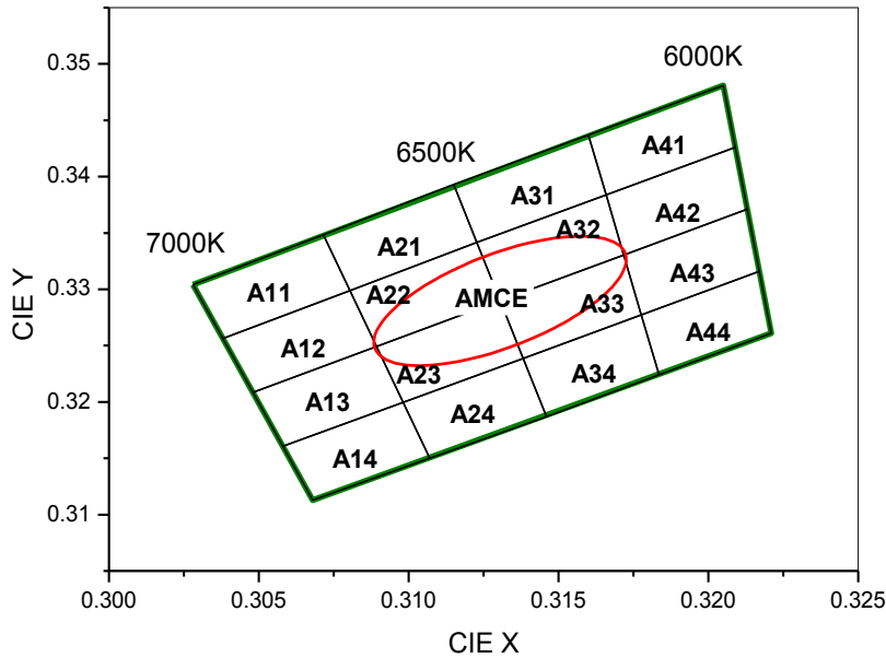
CIE Chromaticity Diagram (Cool white), T_j=25^\circ\text{C} , I_F=65\text{mA}
